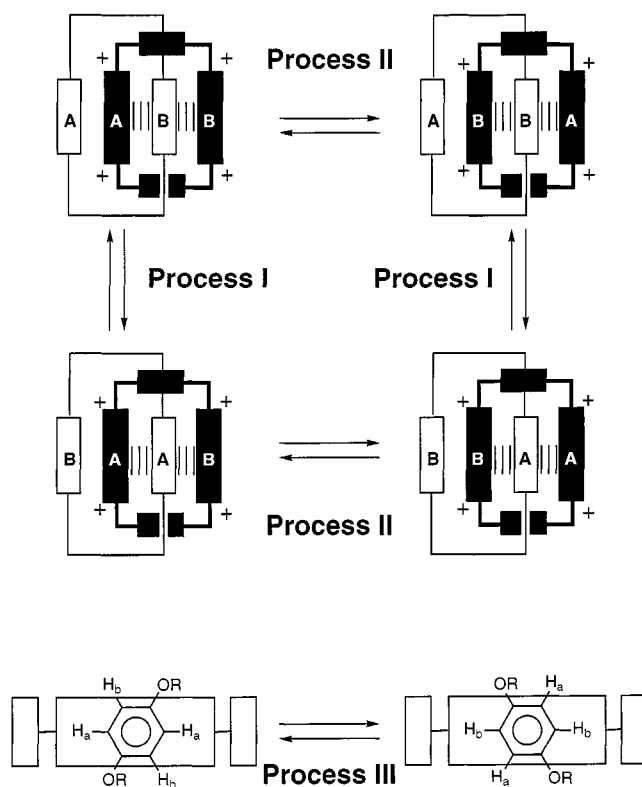
Figure 3. The dynamic processes associated with the [2]catenanes in solution
