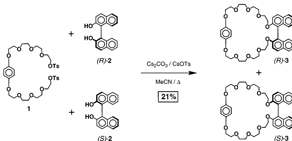
Scheme 1. Synthesis of the crown ethers (R)-3 and (S)-3
