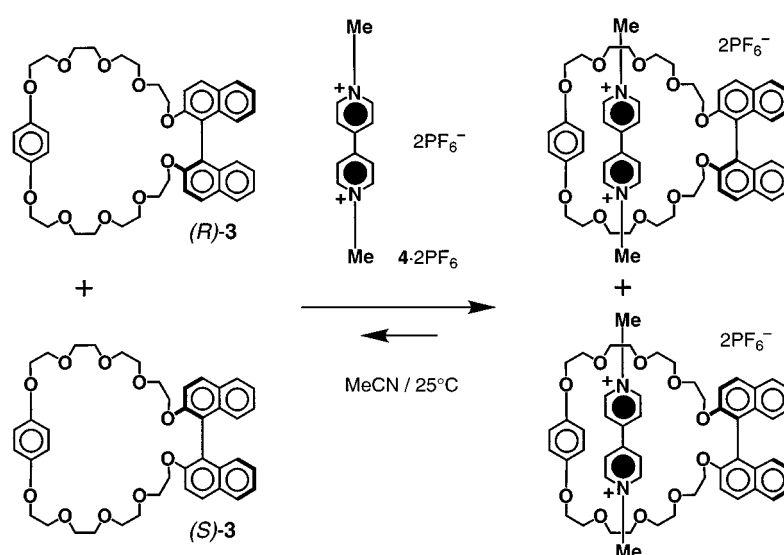
Scheme 2. Complexation of 4 \cdot 2\text{PF}_6 by (R)-3 and (S)-3
