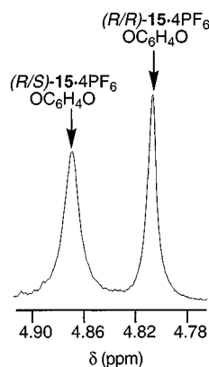
Figure 6. Partial ^1\text{H} -NMR spectrum of a mixture of ( R/S )-15-4PF 6 of ( R/R )-15-4PF 6 recorded in (\text{CD}_3)_2\text{CO} at 323 K
