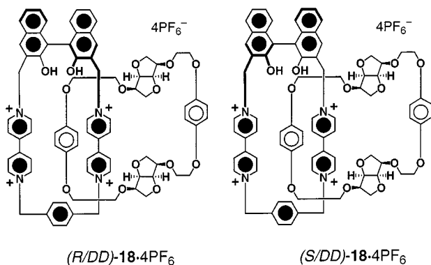
Figure 2. The two diastereoisomers ( R / DD )- 18·4PF 6 and ( S / DD )- 18·4PF 6
