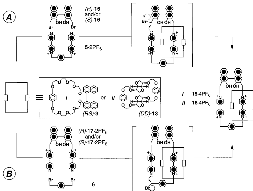
Scheme 6. The routes A and B used to synthesize the [2]catenanes 15·4PF 6 and 18·4PF 6
