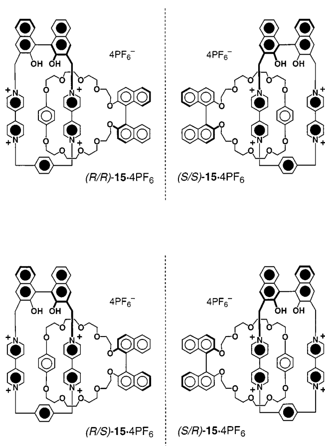
Figure 1. The two pairs of enantiomers associated with the [2]catenanes 15 ·4PF 6
