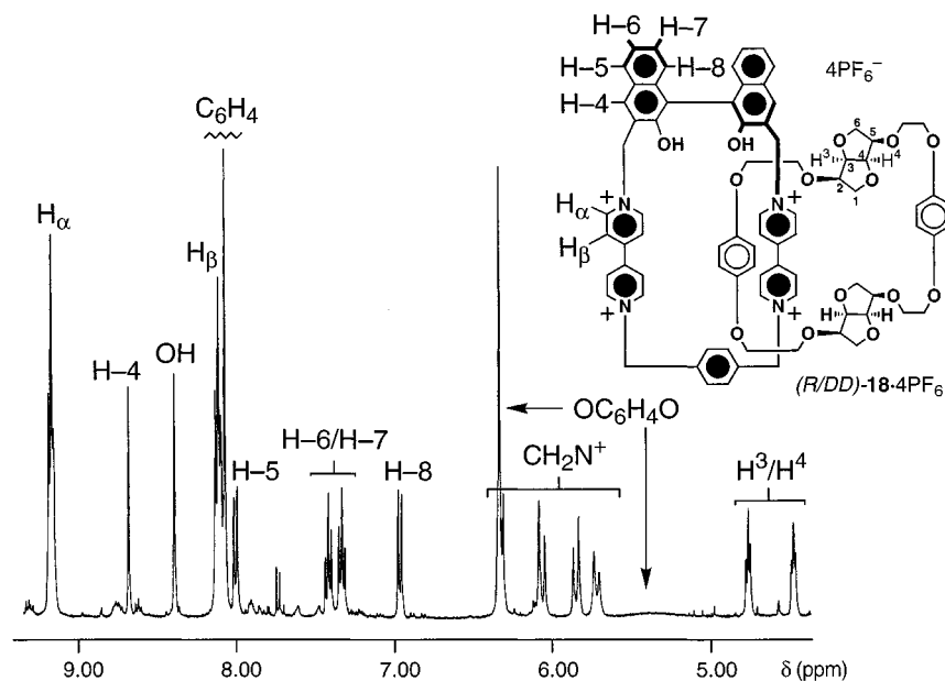
Figure 5. Partial ^1\text{H} -NMR spectrum of the [2]catenane ( R/DD )-18-4PF 6 recorded in (\text{CD}_3)_2\text{CO} at 253 K
