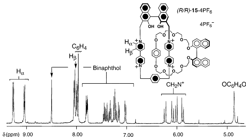
Figure 4. Partial 1 H-NMR spectrum of the [2]catenane ( R/R )-15·4PF 6 recorded in (CD 3 ) 2 CO at 323 K
